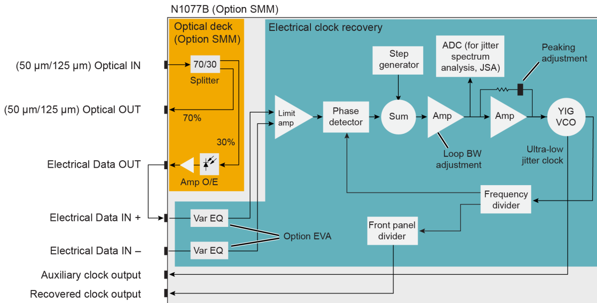
Figure 5. The N1077B with Option SMM combines an integrated 70-30 splitter and an amplified O/E with an instrument grade clock recovery circuit.
