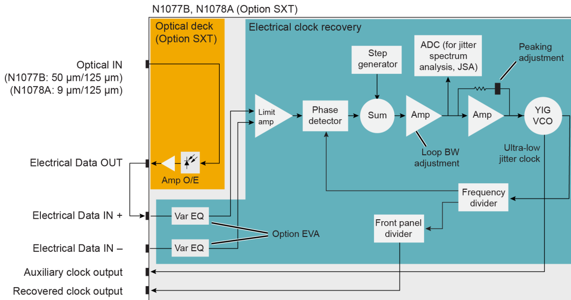
Figure 7. The N1077B and N1078A with Option SXT combine an integrated amplified O/E with an instrument grade electrical clock recovery circuit. The user supplies an external optical splitter as necessary (10-90, 20-80, 30-70, 50-50, etc.).
