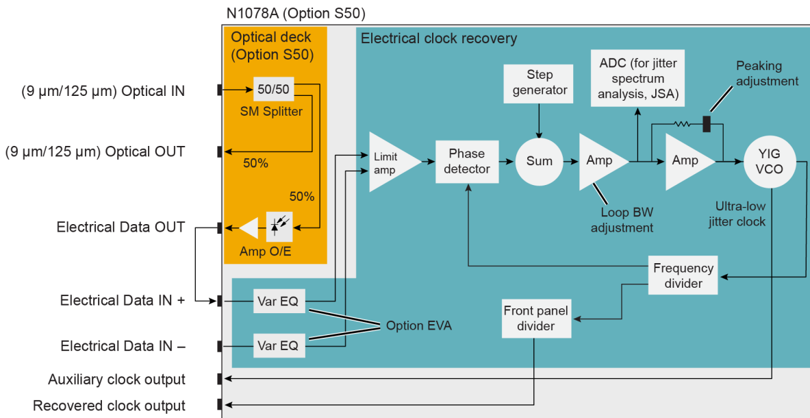
Figure 6. The N1078A with Option S50 combines an integrated 50-50 splitter and an amplified O/E with an instrument grade clock recovery circuit.
