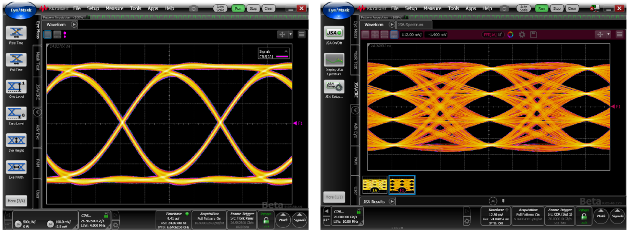
Figure 8. The N107x provides clock recovery capabilities for NRZ (left) and PAM4 (right) signals.
