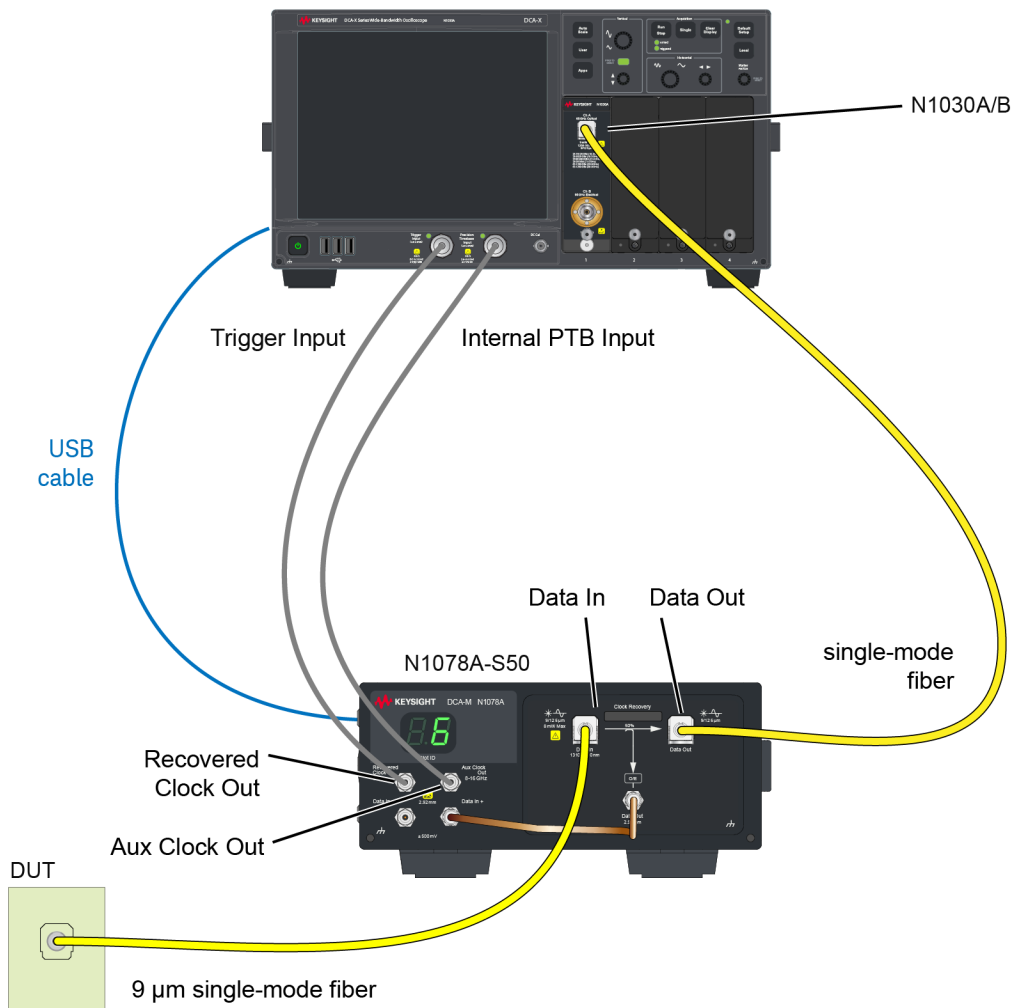
Figure 13. Connection diagram showing an N107x connected to an N1000A DCA-X and N1030A module.
