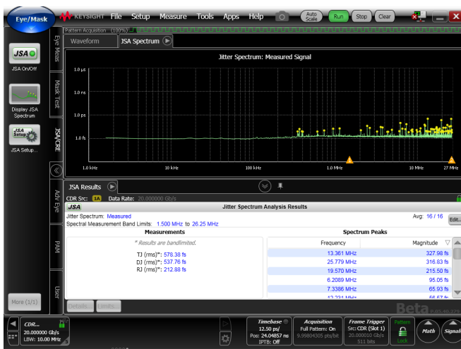
Figure 9. Jitter spectrum analysis (N107xA Option JSA) optimizes Jitter Mode accuracy (N1010100A R&D Package), measures low-frequency jitter (phase noise), and provides insight into the root cause(s) of jitter.
