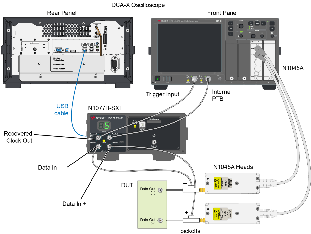
Figure 12. Connection diagram showing an N107x connected to an N1000A DCA-X and remote head modules using high-bandwidth electrical pick-offs (optional accessory).
